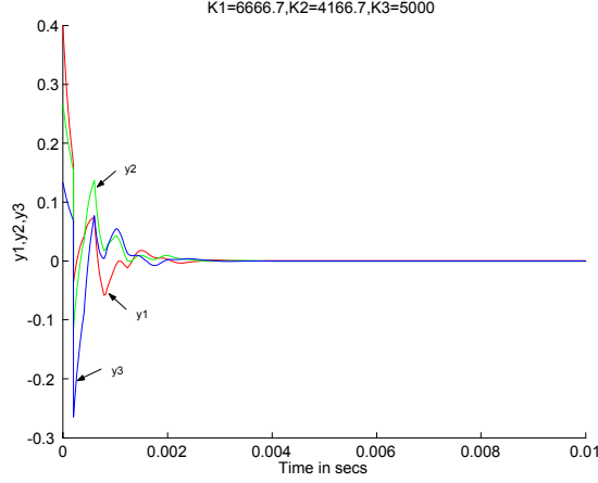
Figure 2: Nonlinear simulation with constant p_{ij} and K1 = 6666.7 ; K2 = 4166.7 ; K3 = 5000
