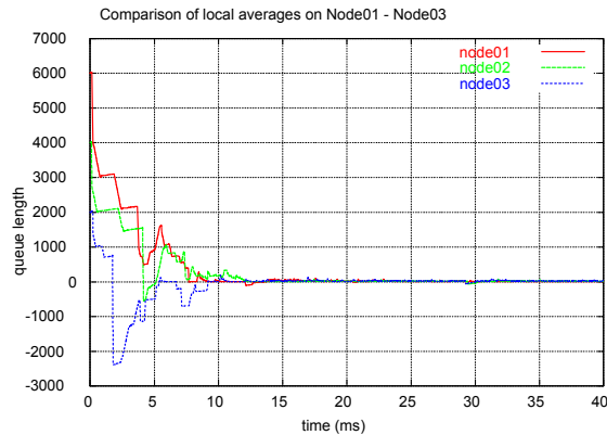
Figure 4: Experimental response of the load balancing algorithm. The average value of the gains are ( K_z = 0.5 ) K_1 = 6667, K_2 = 4167, K_3 = 5000 with constant p_{ij} .
