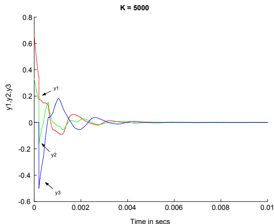
Figure 3: Nonlinear output responses with K = 5000 .
