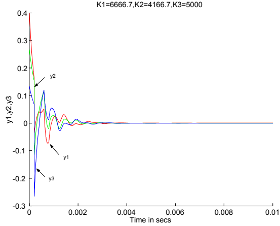
Figure 1: Linear simulation with K1 = 6666.7 ; K2 = 4166.7 ; K3 = 5000
