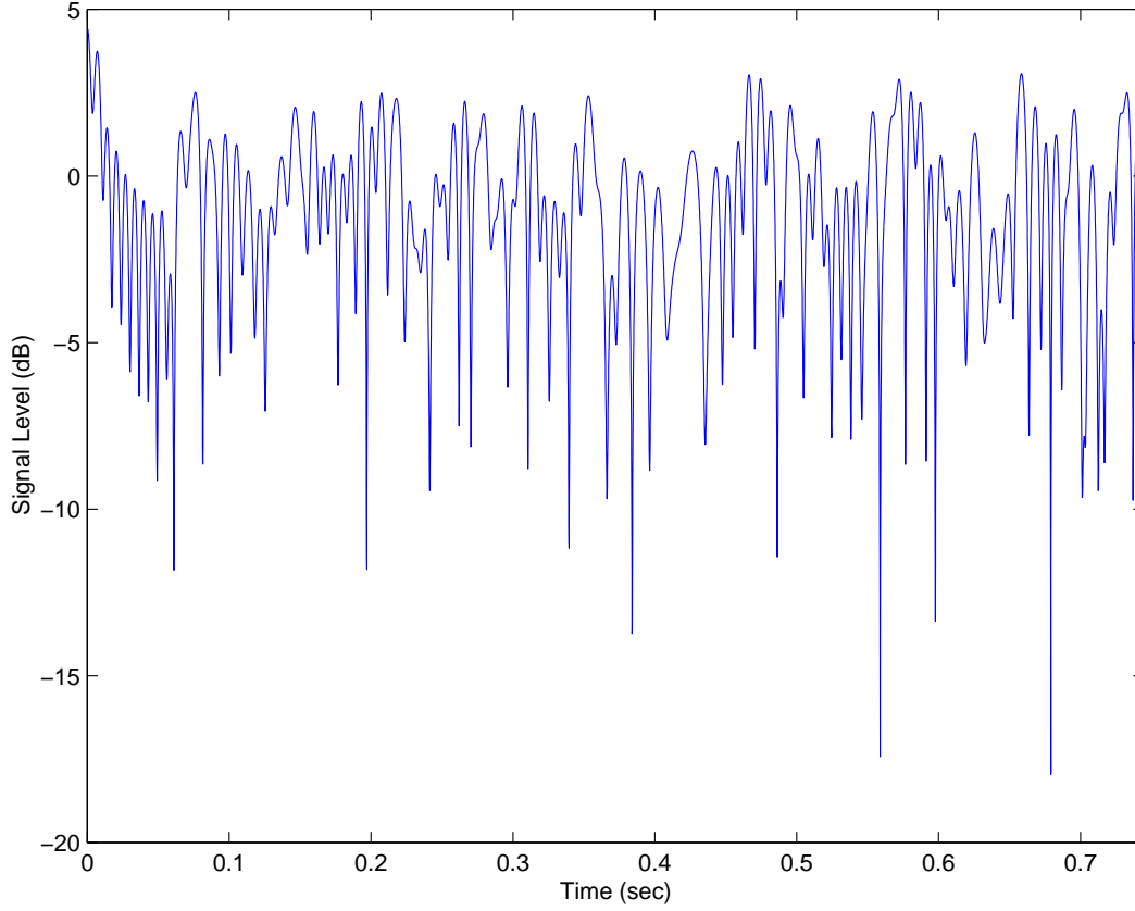
Fig. 2. A typical Rayleigh fading envelope at 845MHz and receiver speed of 100km/hr
