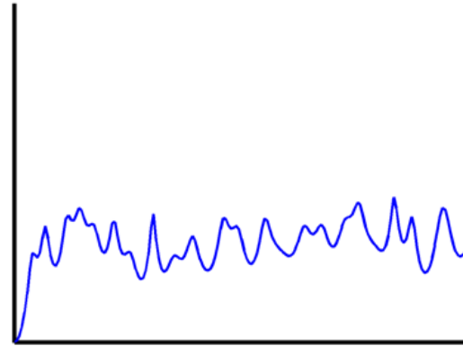
New technique
