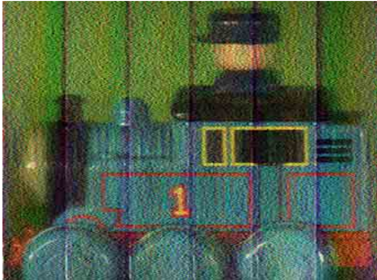
Traditional deblurring
