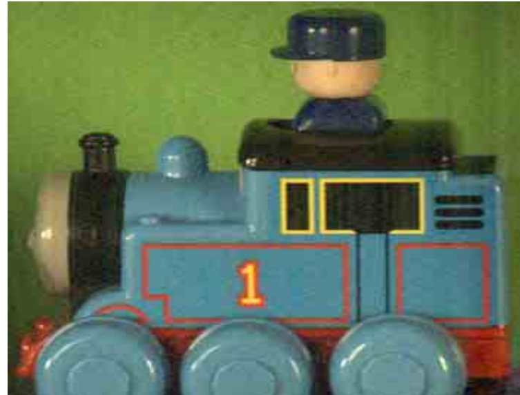
New technique
