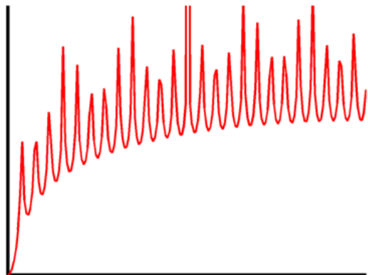
Traditional deblurring
