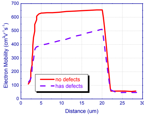
Figure 5. Predicted electron mobility in the GaN vertical JFET. The x-axis is the distance from the source toward the drain.
