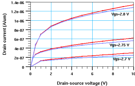
Figure 6. Predicted I-V curve for the 4H-SiC vertical JFET. The dark curves are results for the perfect material. The gray curves include the effects of defects.
