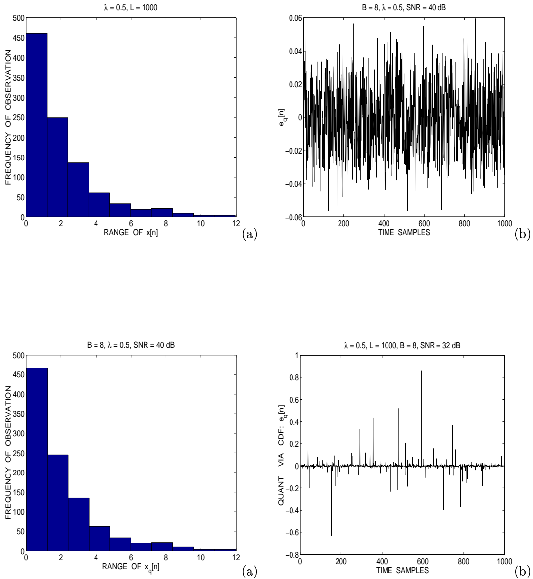
Figure 1: Comparison of the CDF method with nonuniform quantization: (a) Histogram of exponentially distributed input source x[n] , (b) corresponding quantization error e_q[n] via Lloyd Max quantization (c) histogram of x_q[n] from the CDF method, (d) corresponding output quantization error e_{\text{out}}[n]
