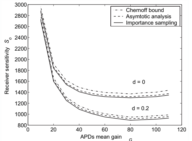
Fig. 2: Receiver sensitivity as a function of the APD's mean gain \mu_G for d = 0 and d = 0.2 . It is assumed that \sigma^2 = 8 \times 10^6 and that each incident photon results in a primary electron.
