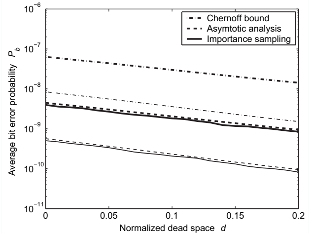
Fig. 1: Average bit-error probability as a function of the normalized dead space. For each method, thick and thin curves correspond to mean numbers of primary electrons \lambda of 4000 and 4500, respectively. The variance of the Gaussian thermal noise is assumed as \sigma^2 = 3.6 \times 10^7 [1].
