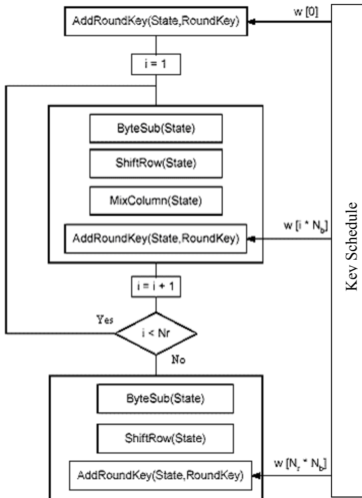
Figure 4. Encryption Process [6]
