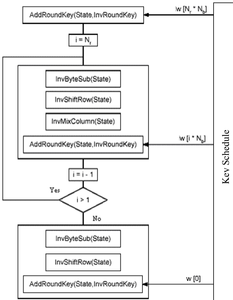
Figure 12. Decryption Process [6]
