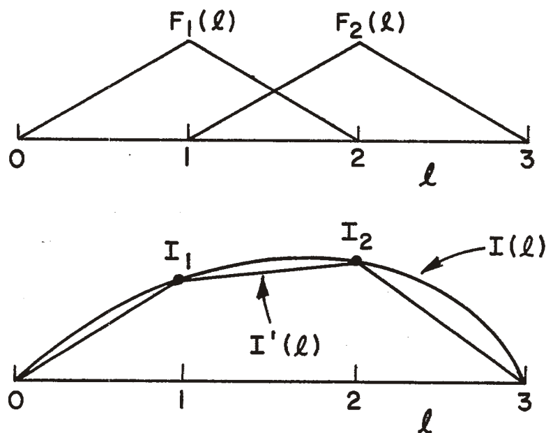
Fig. 2. The expansion functions F_1(\ell) and F_2(\ell) , the current distribution I(\ell) and the two-mode approximation I'(\ell) .
