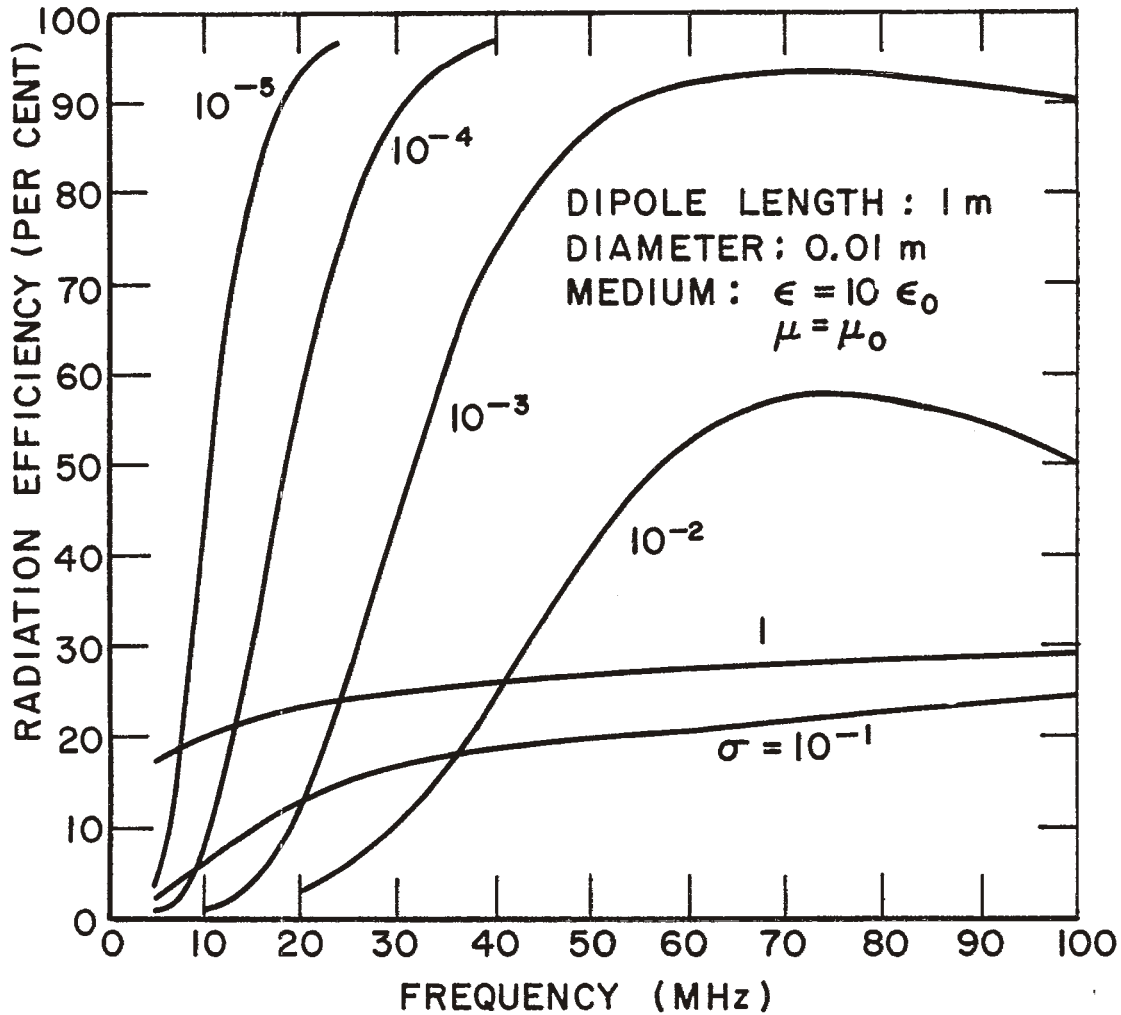
Fig. 4. Radiation efficiency of uninsulated perfectly-conducting center-fed linear dipole in a homogeneous medium with conductivity \sigma in mhos/m.
