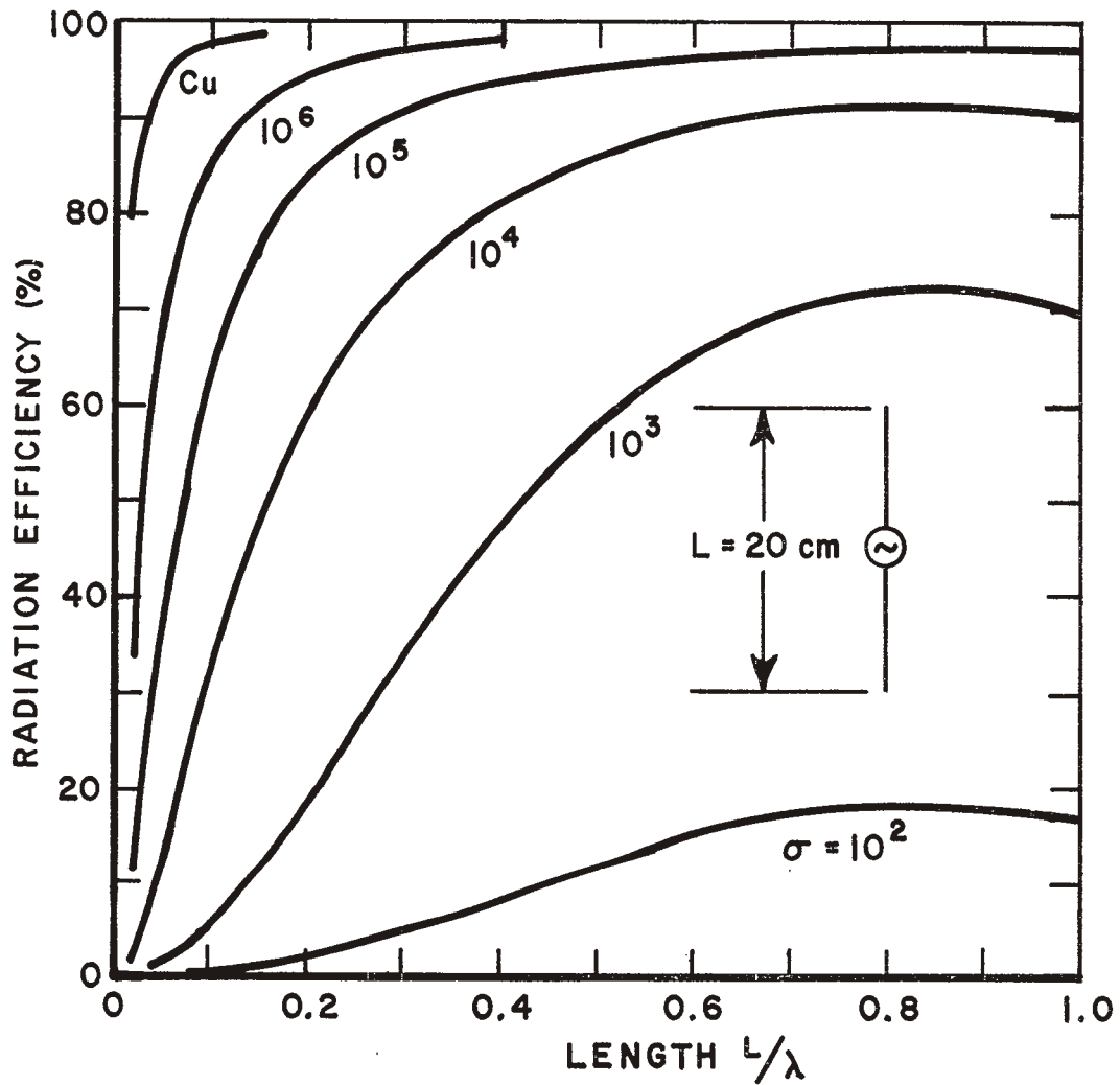
Fig. 8. Radiation efficiency of center-fed dipole in free space. The parameter is the conductivity in mhos per meter. Wire diameter: 1/16 inch solid.
