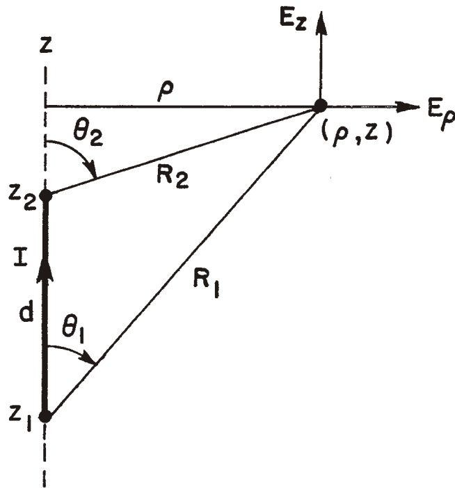
Fig. 12. An electric line source on the z axis and the observation point at (\rho, z) .
