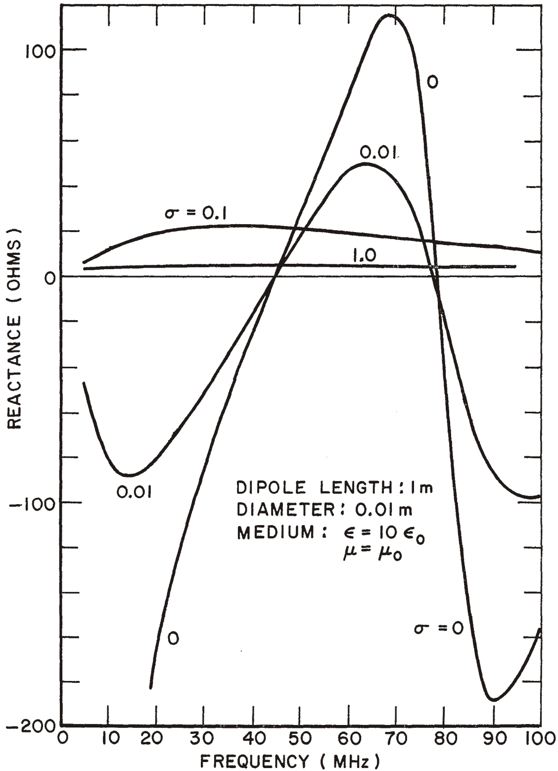
Fig. 6. Reactance of uninsulated perfectly-conducting center-fed linear dipole in a homogeneous medium with conductivity \sigma in mhos/m.
