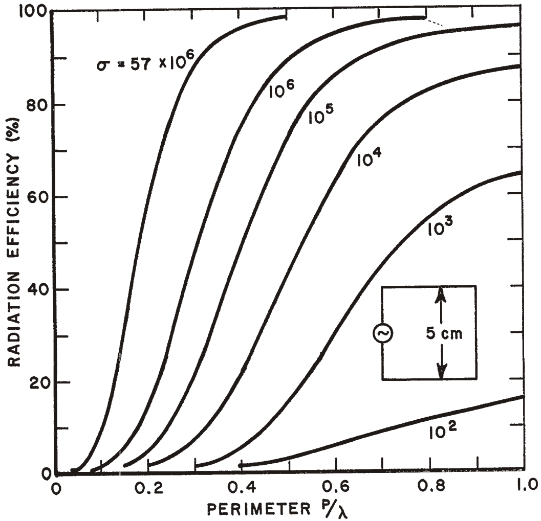
Fig. 9. Radiation efficiency of square loop antenna in free space. The parameter is the conductivity in mhos per meter. Wire diameter: 1/16 inch solid.
