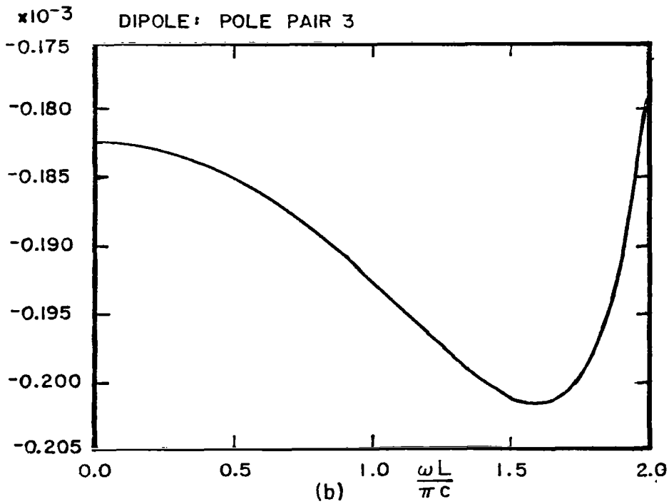
Figure 4. (a) Real part characteristic of an unmodified pole-pair module for the dipole antenna, and (b) fragment of (a).
