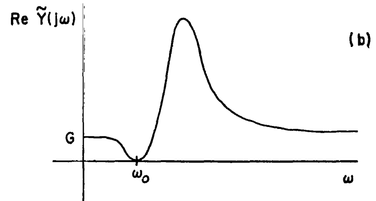
Figure 27. Real part characteristic of a modified pole-pair module typical for the dipole and loop antennas. (a) Before padding, and (b) after padding.
