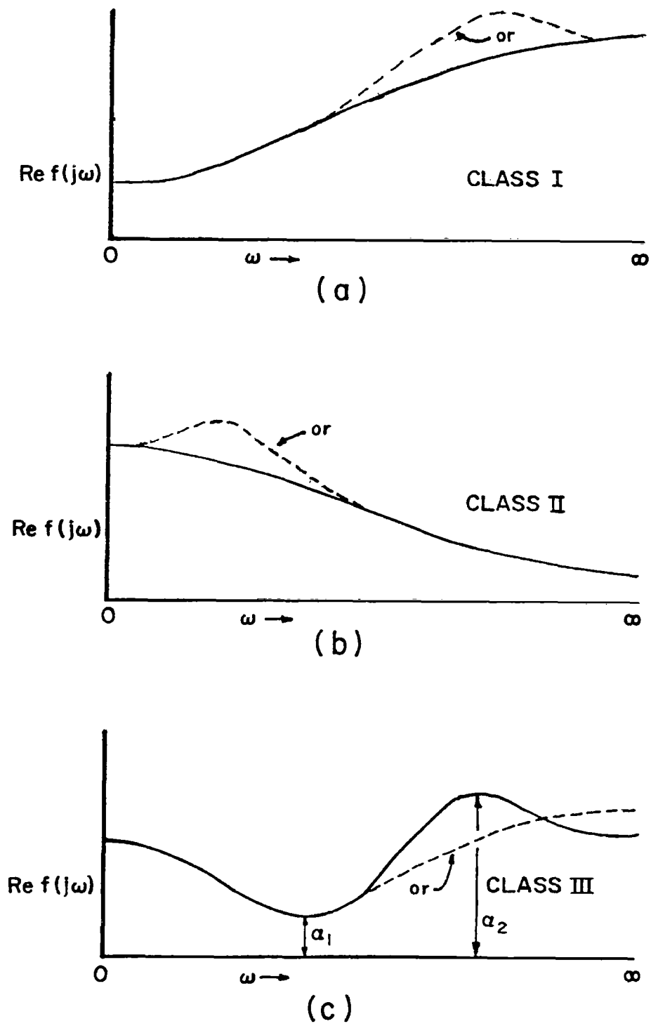
Figure 3. Real part characteristics of three classes of PR biquadratic functions.
