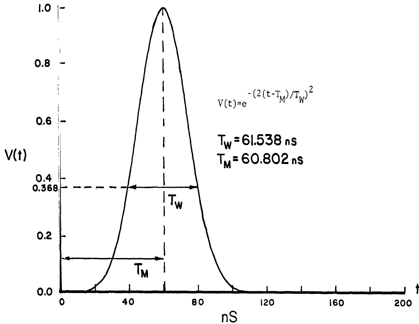
Figure 12. Gaussian pulse used in transient analyses.
