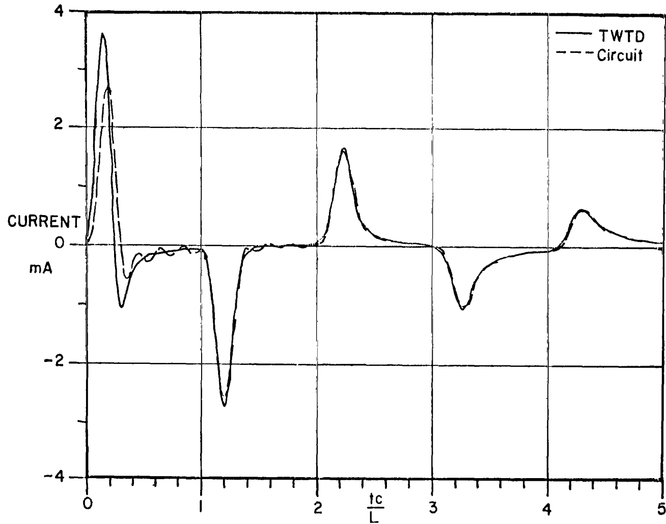
Figure 31. Transient response of the lumped circuit (Figure 30) and the result of TWTD program analysis.
