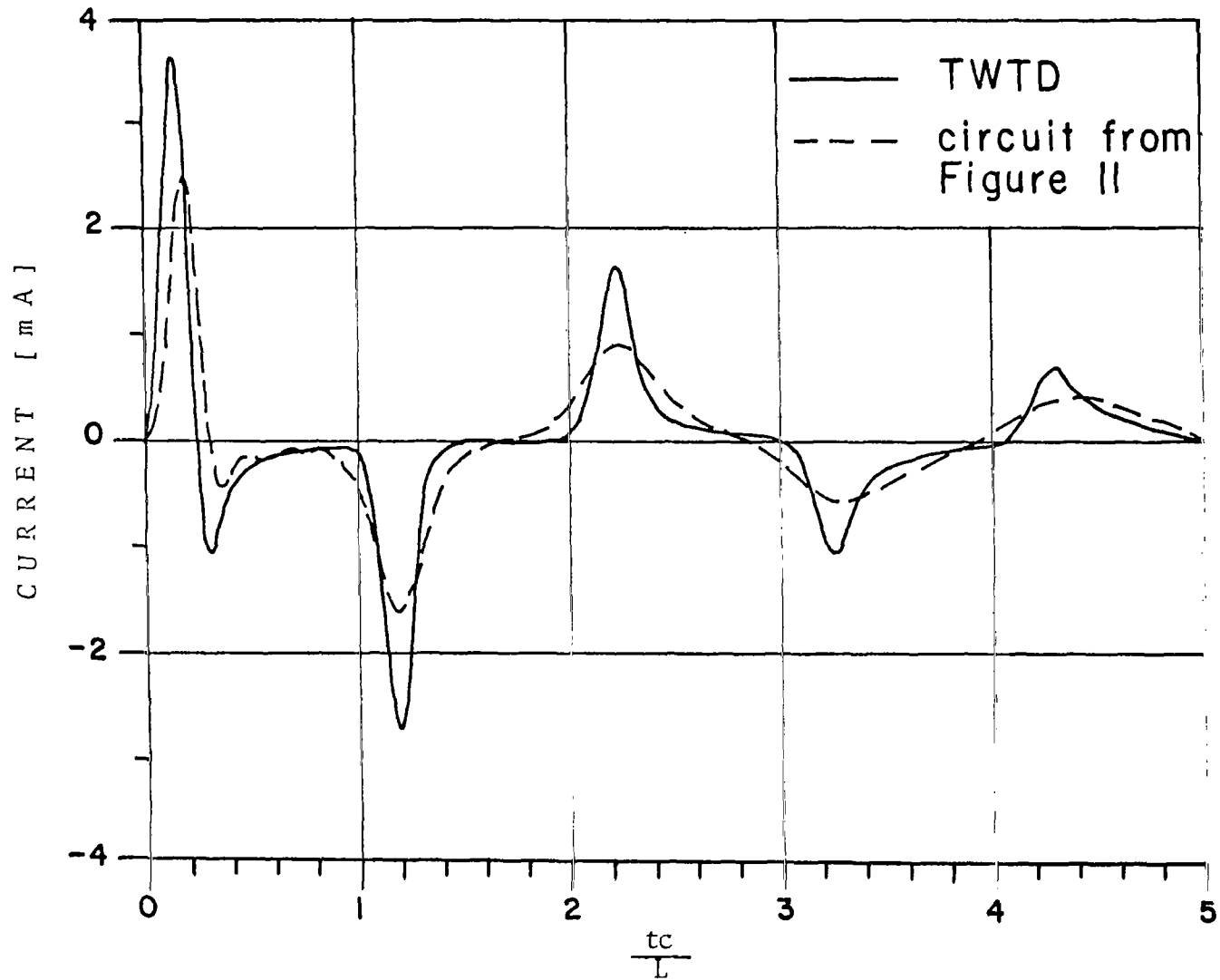
Figure 13. Transient response of the lumped circuit (Figure 11) and the result of the TWTD program analysis.
