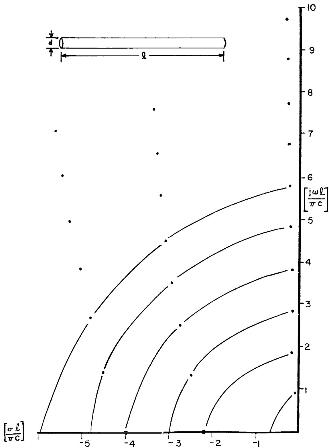
Figure 1. Natural frequencies of the straight wire with L/d = 100 .
