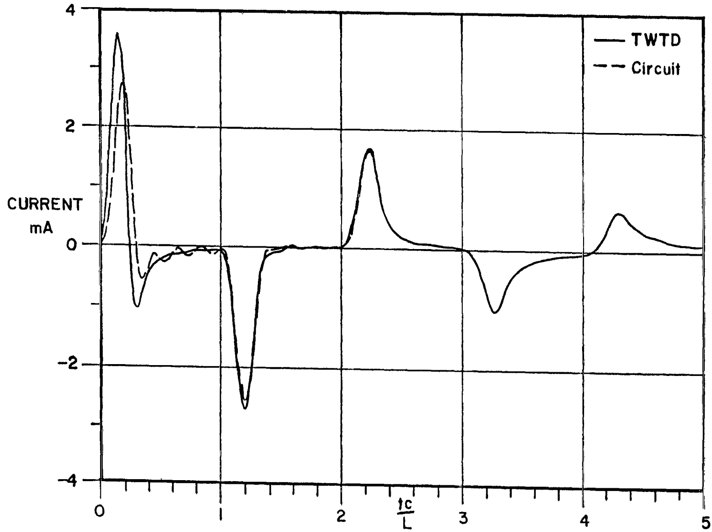
Figure 19. Transient response of the lumped circuit (Figure 18) and the result of TWTD program analysis.
