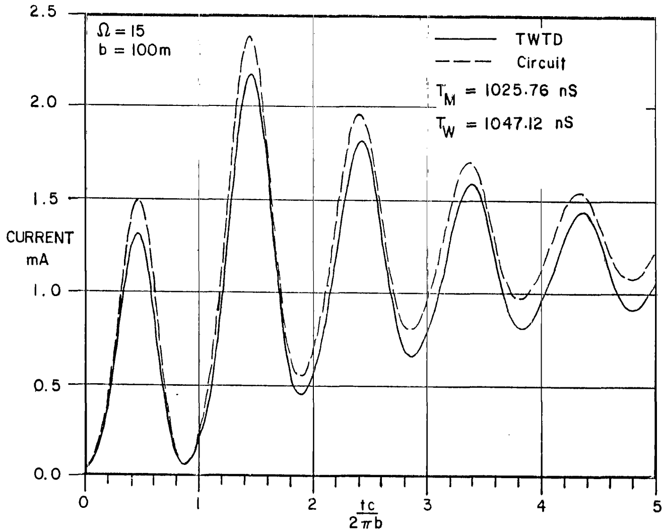
Figure 31B. Transient response of the lumped circuit (Figure 31A) and the result of the TWT program analysis.
