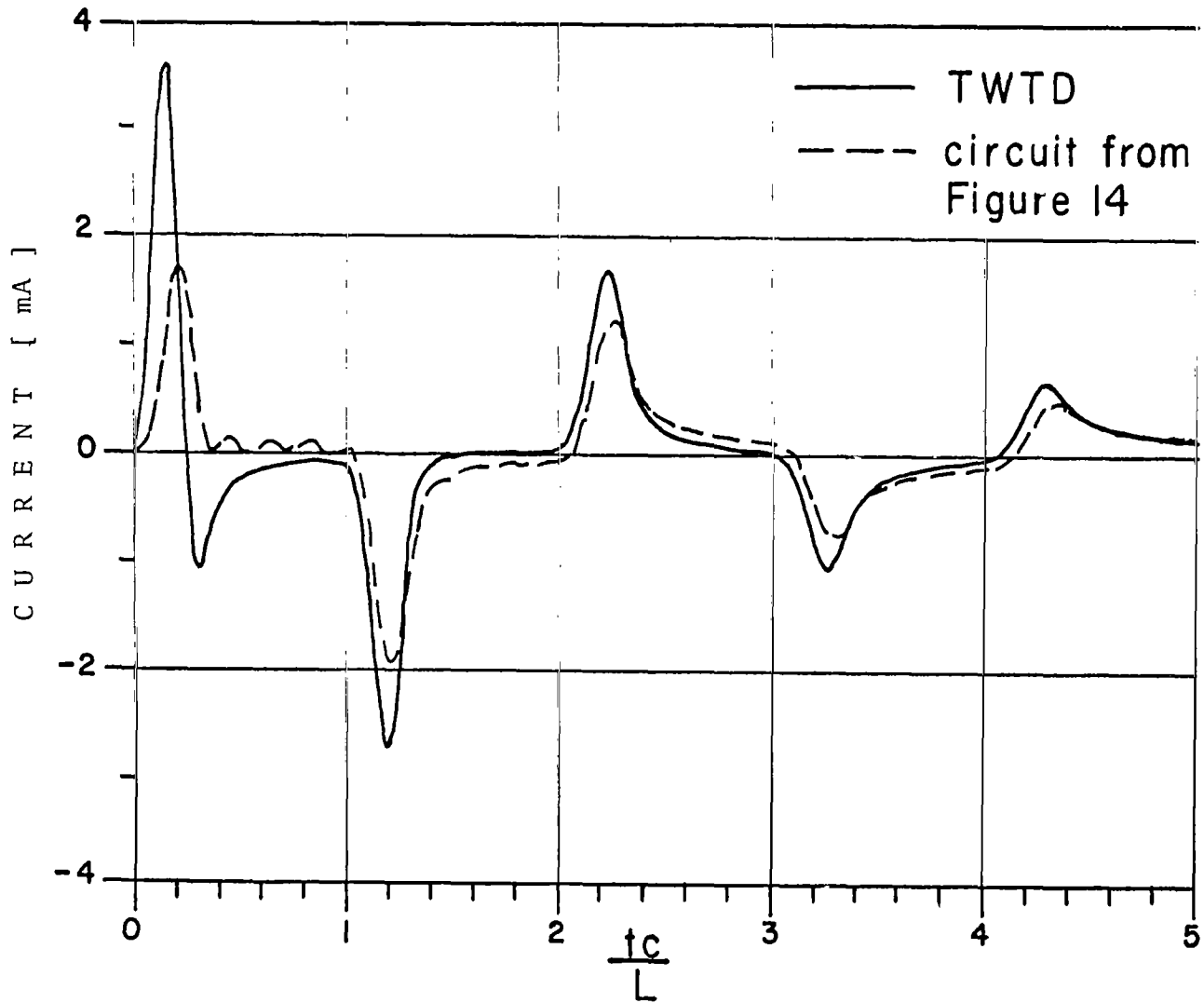
Figure 15. Transient response of the lumped circuit (Figure 14) and the result of the TWTD program analysis.
