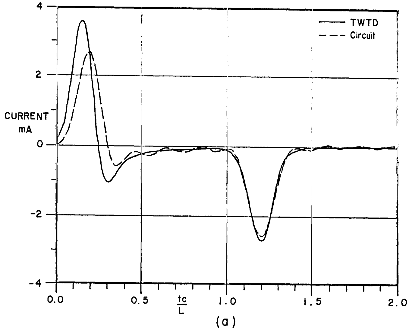
Figure 44. Early time response of the equivalent network for the dipole antenna (Figure 30). (a) Without correction, and (b) with 70pF shunt capacitor.
