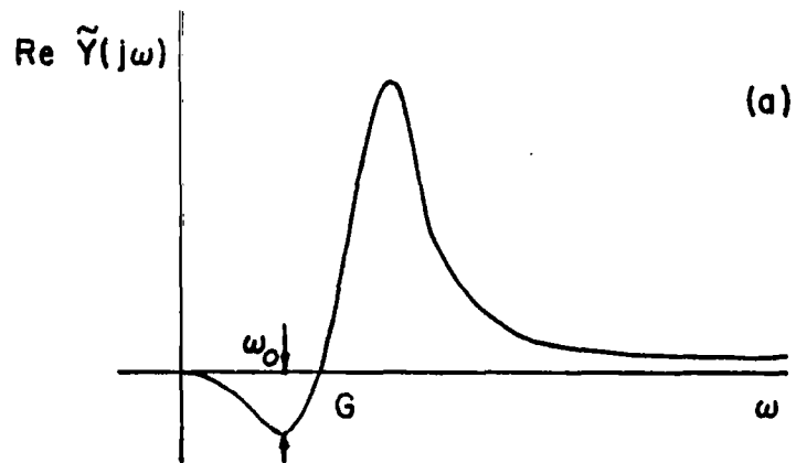
Figure 27. Real part characteristic of a modified pole-pair module typical for the dipole and loop antennas. (a) Before padding, and (b) after padding.
