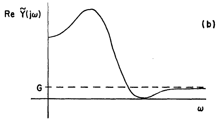
Figure 28. Real part characteristic of a pole-pair module for a hypothetical structure. (a) Before padding, and (b) after padding.
