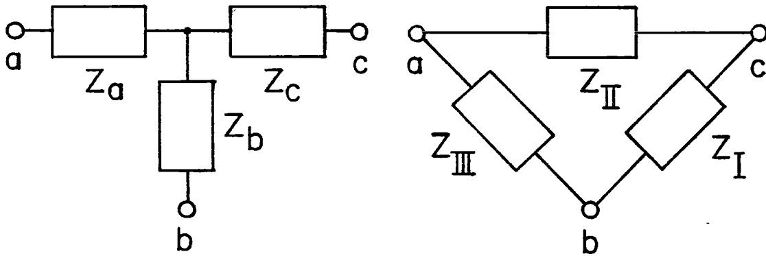
Figure 23. Illustration of the T-delta transformation.
