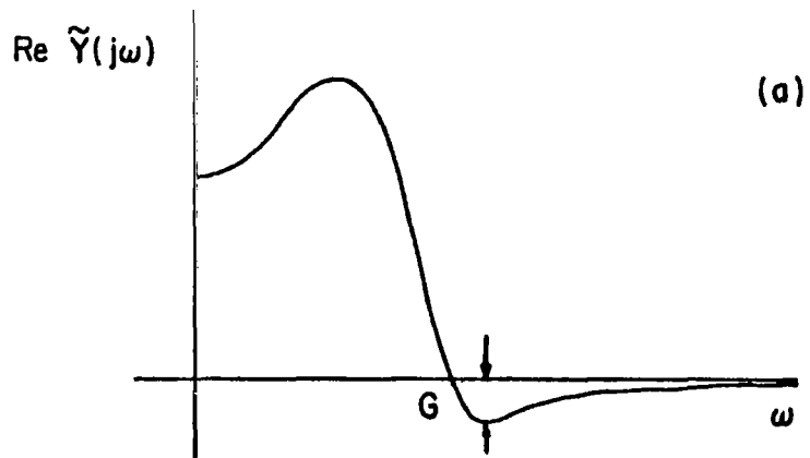
Figure 28. Real part characteristic of a pole-pair module for a hypothetical structure. (a) Before padding, and (b) after padding.
