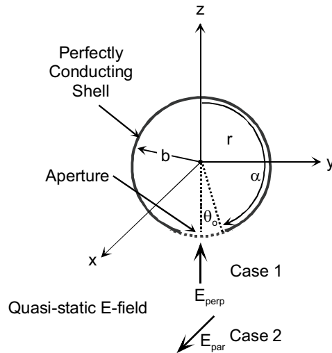
Figure 12. Geometry of a thin, perfectly conducting sphere having a circular aperture and illuminated by a quasi-static E-field.
