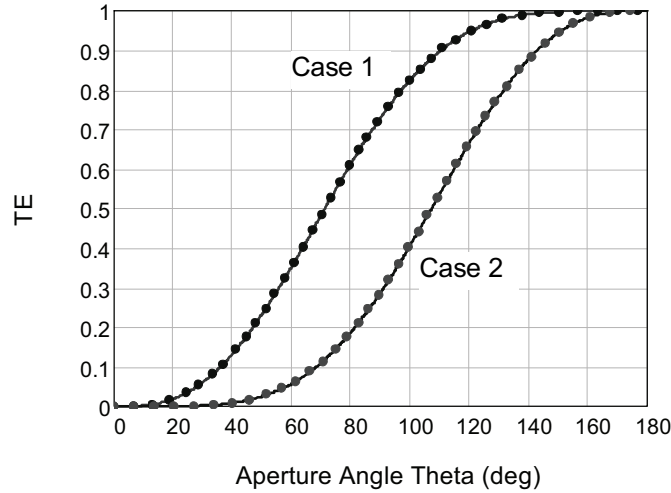
Figure 13. Plot of the E-field transfer function at the center of the spherical enclosure as a function of the aperture half-angle \theta_0 , for Case 1 ( E in z -direction) and Case 2 ( E in x -direction). Dots represent Casey's results, solid lines are for the present analysis
