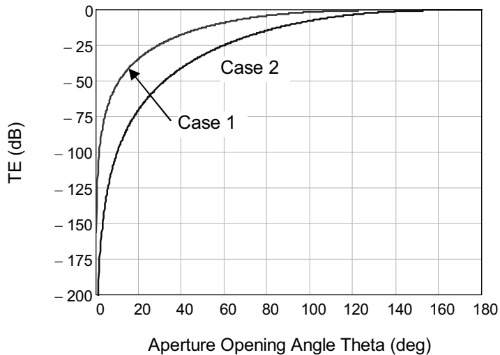
Figure 14. Plots of the E-field transfer function (expressed in dB) at the center of the sphere, as a function of the aperture angle \theta_0 .
