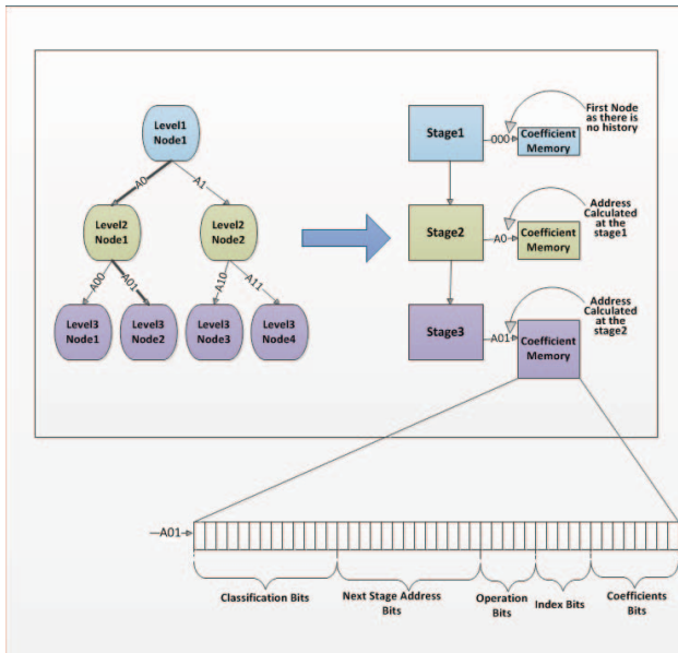
Fig. 2: Decision Tree Stages
