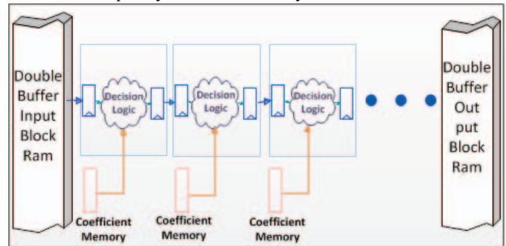
Fig. 3: Decision Tree Classification Subsystem
