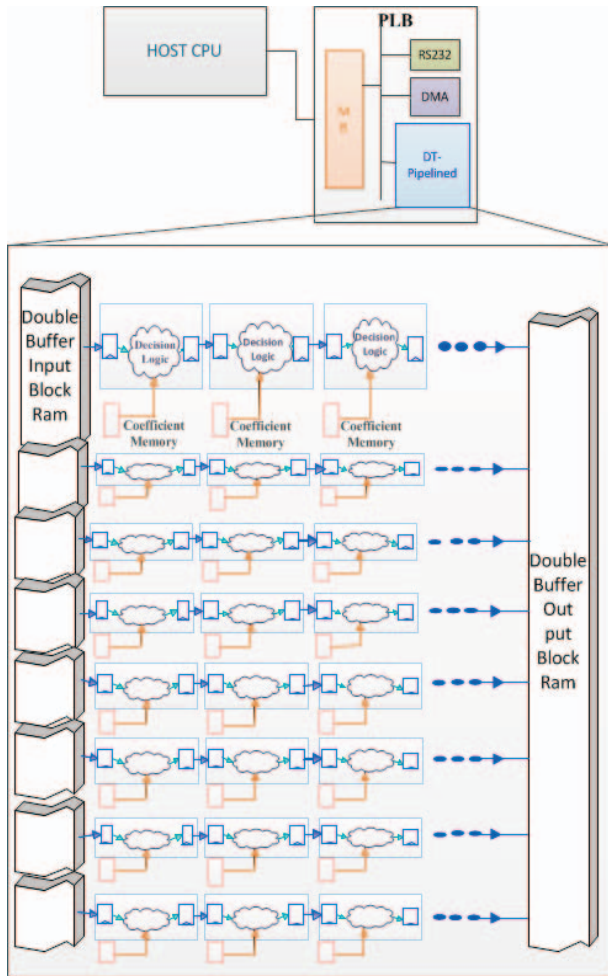
Fig. 5: Parallel and Pipelined Decision Tree Engine
