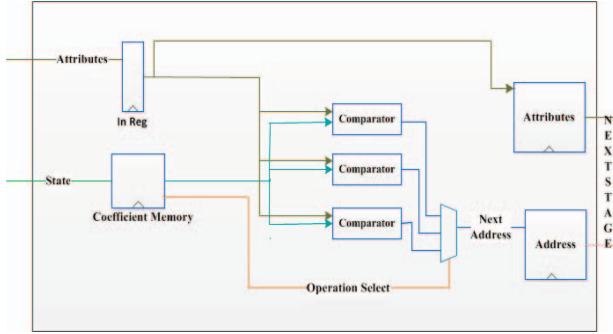
Fig. 4: RTL level Block Diagram of Hardware Module
