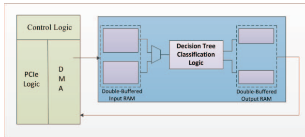
Fig 6: Streaming Architecture
