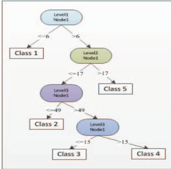
Fig 1: Decision Rules in form of Decision Tree
